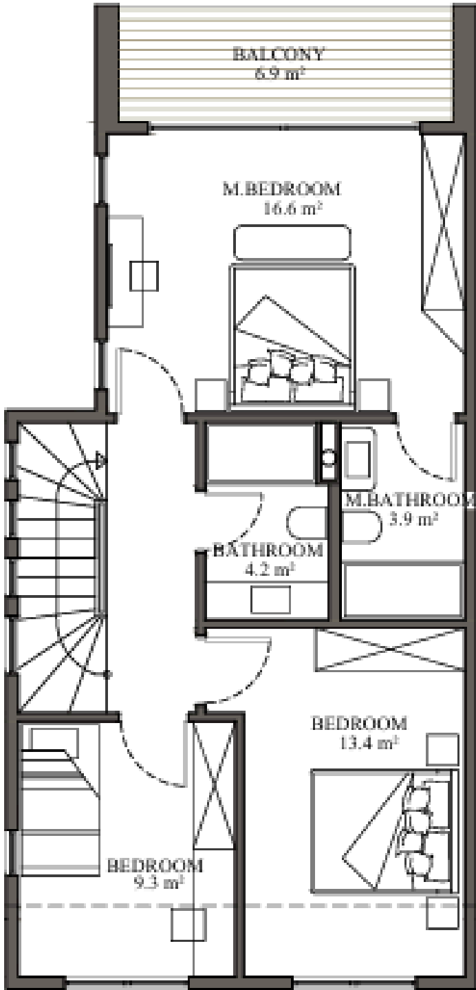
(Alternative ) 1.st Floor Plan Area:70.5 m²
