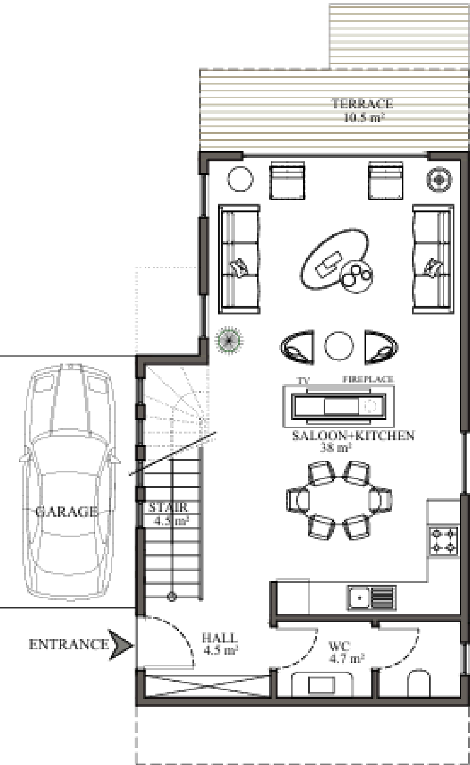
Ground Floor Plan Area:58.5 m²
