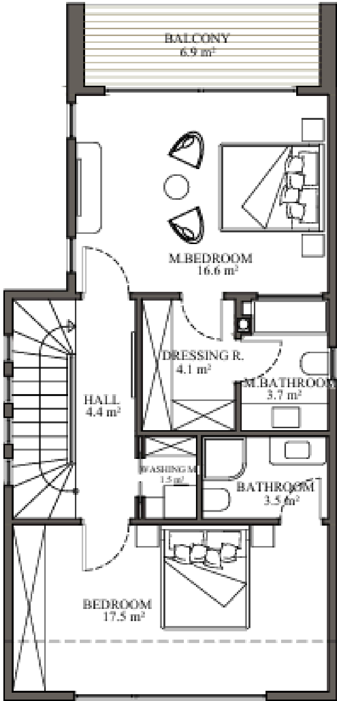
1.st Floor Plan Area:70.5 m²
